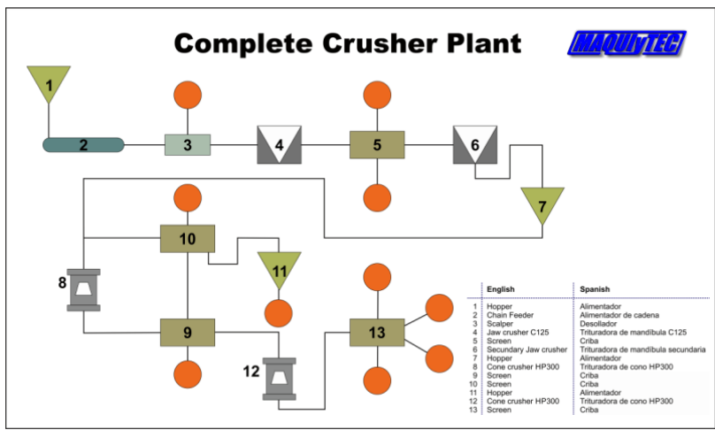
Complete METSO Crusher Plant
